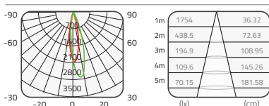
CREE 9W±10% 3000K 20° Ra80
