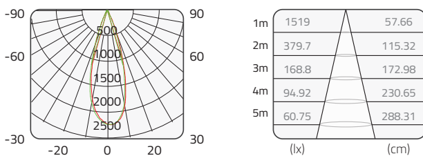
Luminus 8W±10% 3000K 36° Ra90
